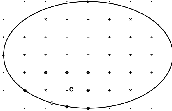
Figure 1: An Ellipse embedded in the grid. + - calculated nodes, x - edge nodes, . - exterior nodes. The circles are the 8 neighbors of the calculated node C
