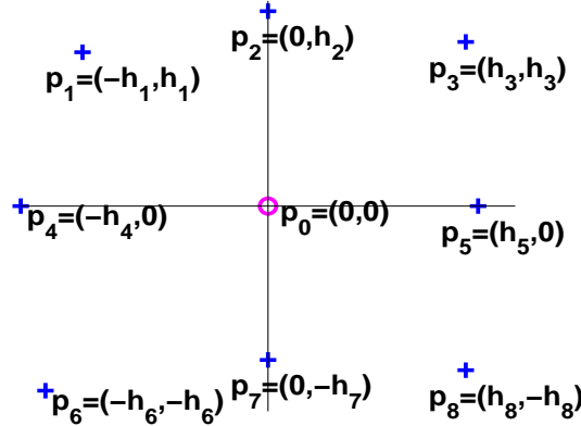
Figure 2: The 8 neighbors
